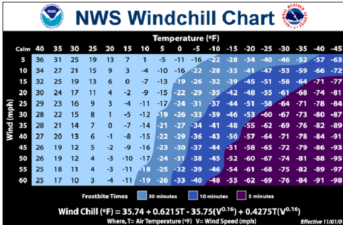
Figure 5.4.6-3. NWS Wind Chill Index
