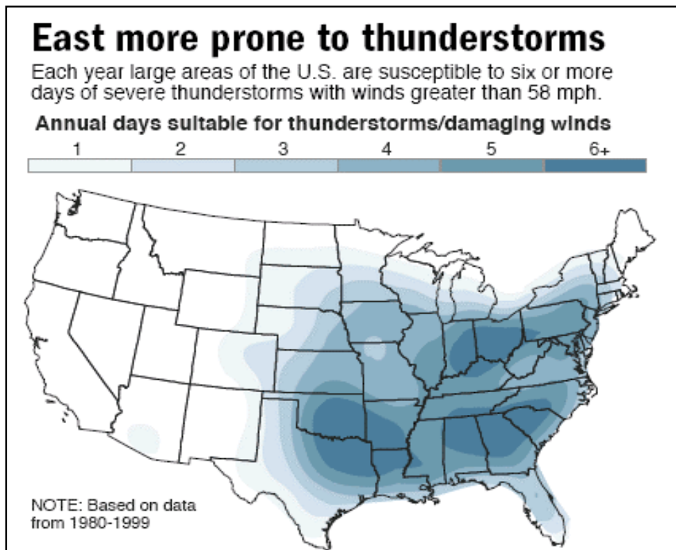
Figure 5.4.6-4 Annual Days Suitable for Thunderstorms/Damaging Winds
