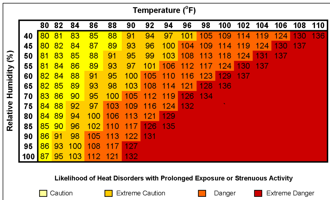
Figure 5.4.6-1. NWS Heat Index Chart
